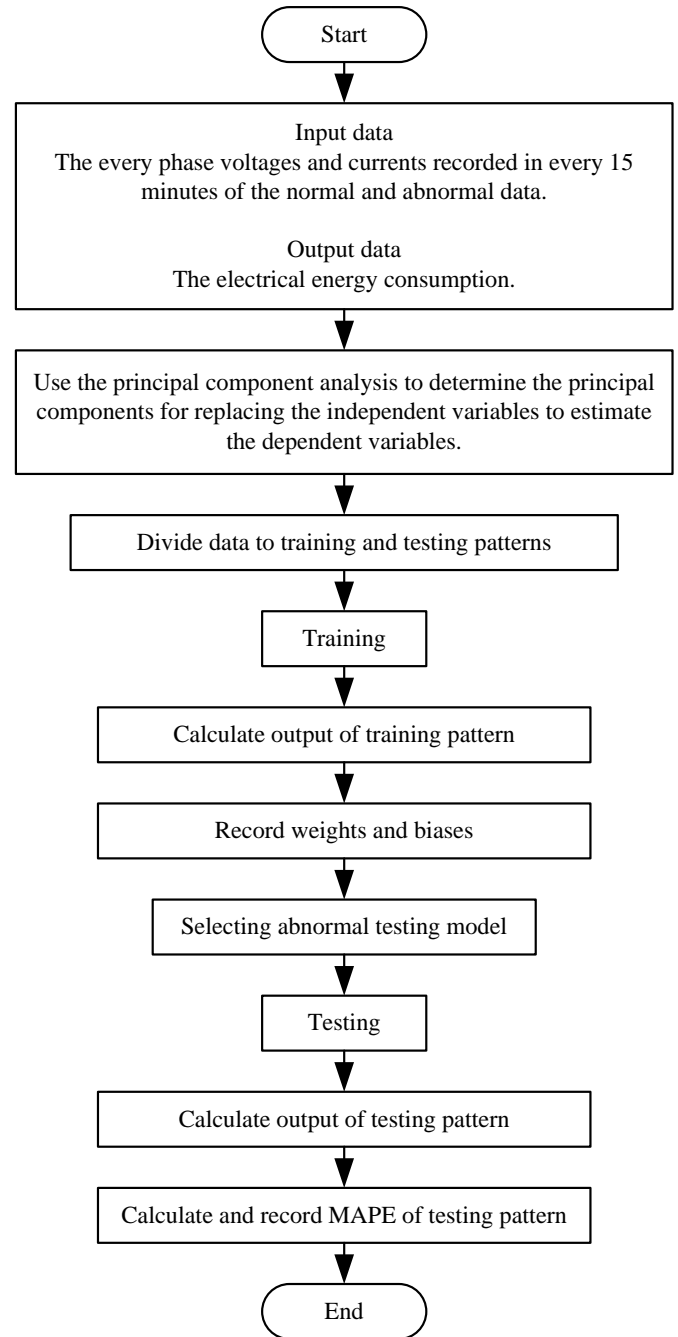
Figure 3. Flowchart diagram for the proposed estimation.
